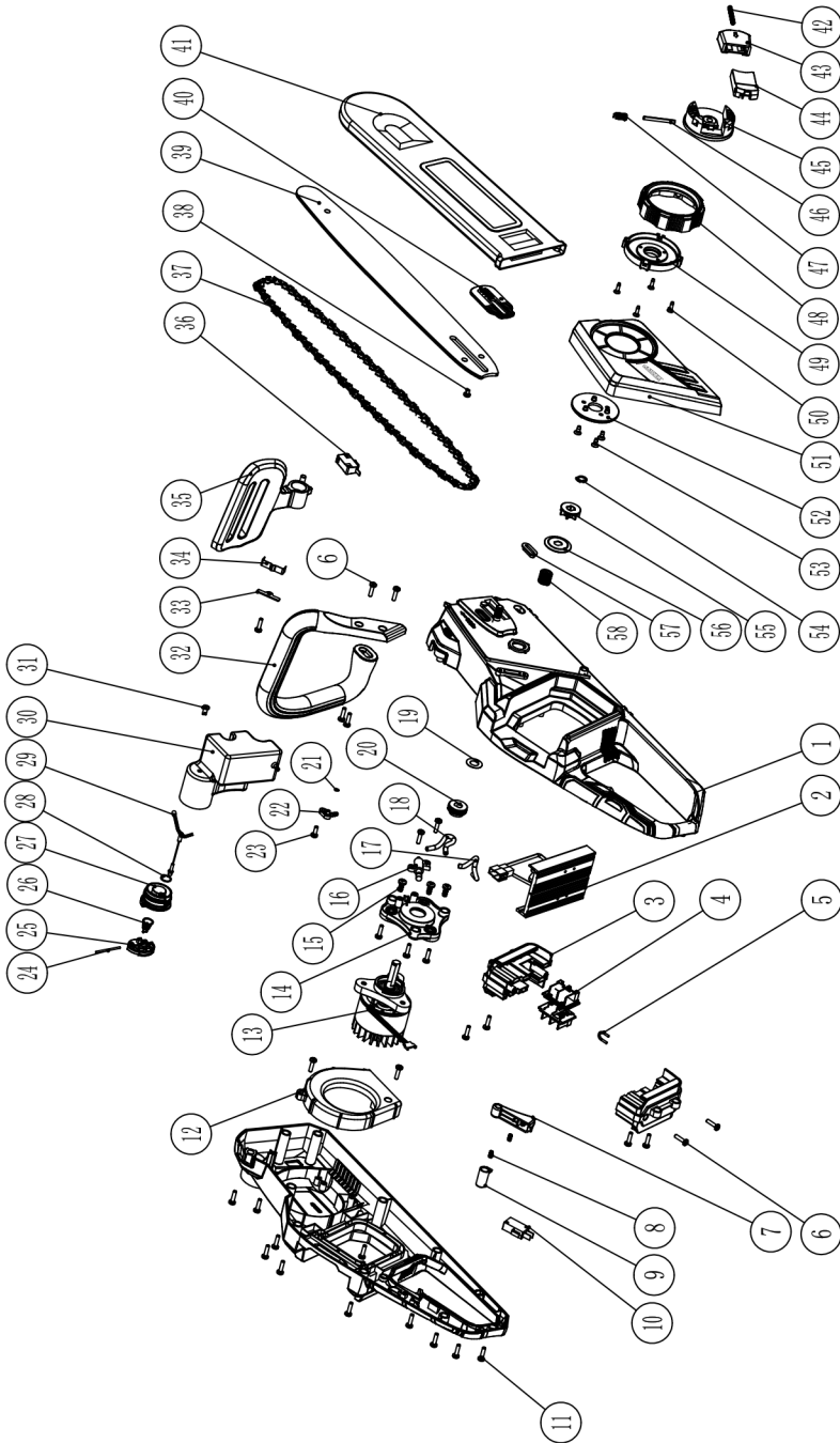
Exploded Drawing of Cordless chain saw brushless RDP-SBCS20 Art. No. 030155.
